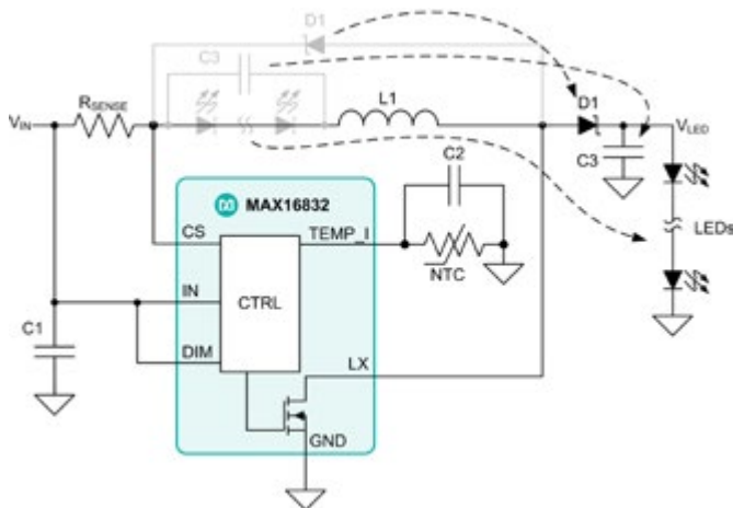
Figure 3: Change topology from high-side buck to boost just requires some rearrangement of the external components.
