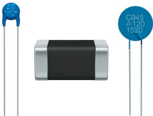
Figure 4: EPCOS protective component for power supplies From left to right: Disk varistor for overvoltage protection at the power input and CeraDiode® for protecting the output, PTC for overcurrent protection at the power input.
