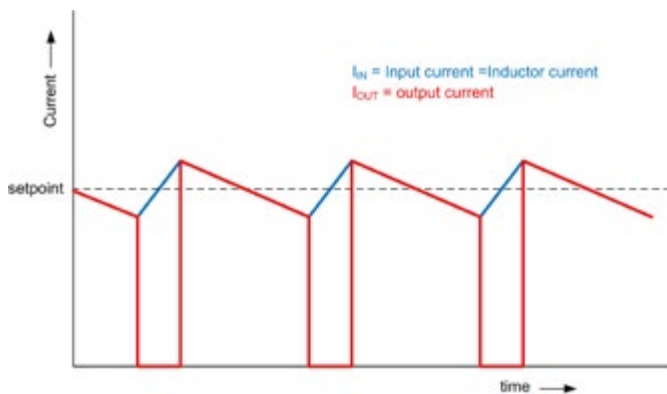
Figure 4: When configured as a hysteretic boost LED driver, the input current is regulated rather than the LED current, as shown by the waveforms for the input and output currents.
