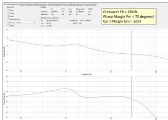
Figure 6: We have used WDS to design a digital power supply with similar specification
