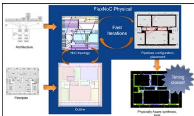
Picture 7: Block Diagram of FlexNoC
