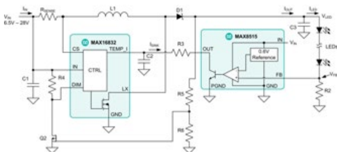
Figure 8: Over-voltage protection is needed when an LED fails open circuit, thus allowing C3 to become charged beyond the maximum rating of the IC.
