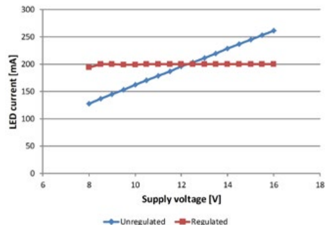
Figure 9: LED current versus input voltage with (red) and without (blue) additional regulation shows the output current's sensitivity to the value the input voltage.
