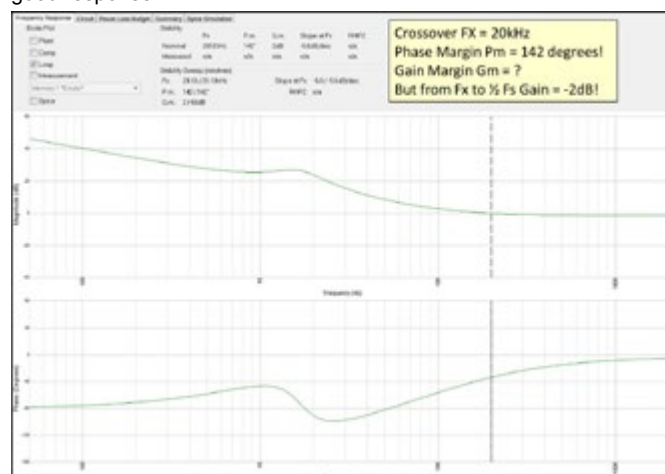
Figure 5: We are only 2dBs below the 0dB point
