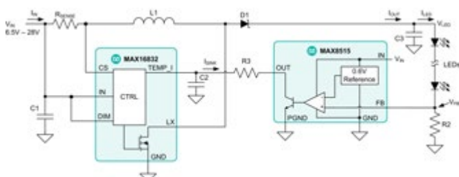
Figure 5: An additional circuit based on the MAX8515 shunt regulator can be used to improve LED current regulation, if needed.
