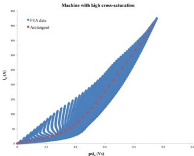
Figure 3: i_q as a function of \psi_q for a machine with heavy cross-saturation
