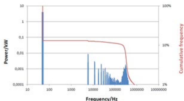
Figure 2: VFD power spectrum
