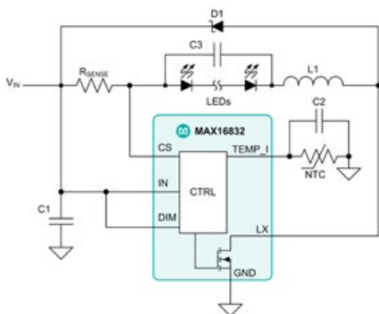
Figure 1: Typical application circuit of the MAX16832 as a buck-converter LED driver
