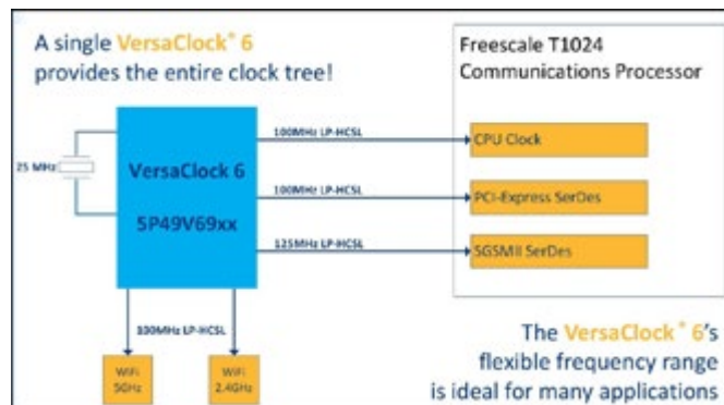
Picture 12: VersaClock 6 programmable Clock Generator
