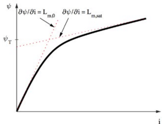
Figure 2: Flux vs Current for a saturable machine based on an arctangent function
