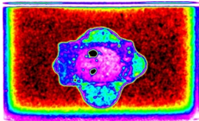
Figure 4: Black features in the die attach of this TO220 device are voids.
