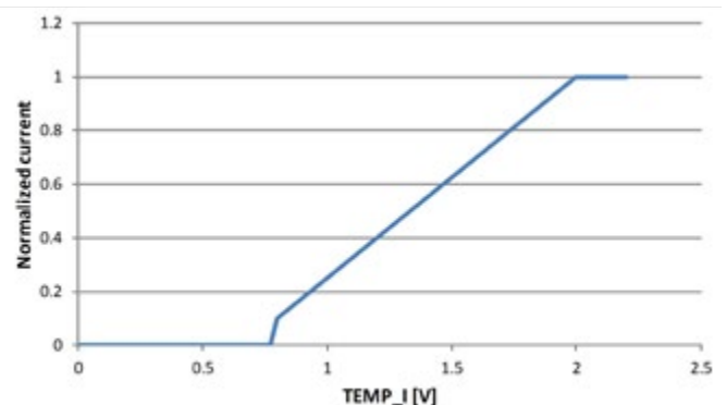
Figure 6: The MAX8515 manages the sinking and sourcing, as seen in the relation between voltage on TEMP_I and input-current set point.
