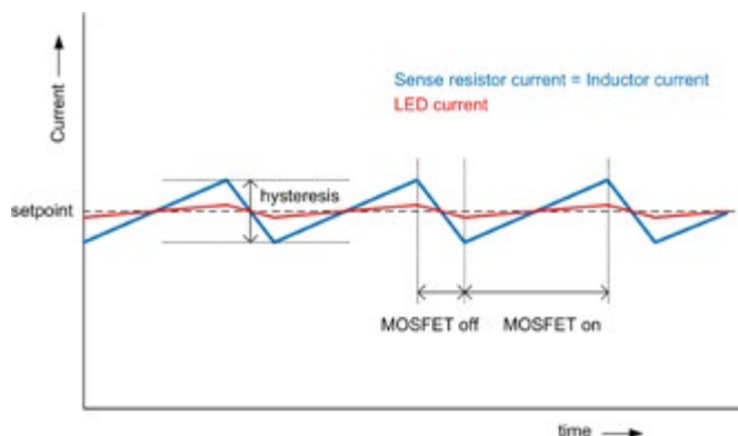
Figure 2: The current waveform of the hysteretic buck LED driver has a sawtooth LED current due to self-induced oscillation.
