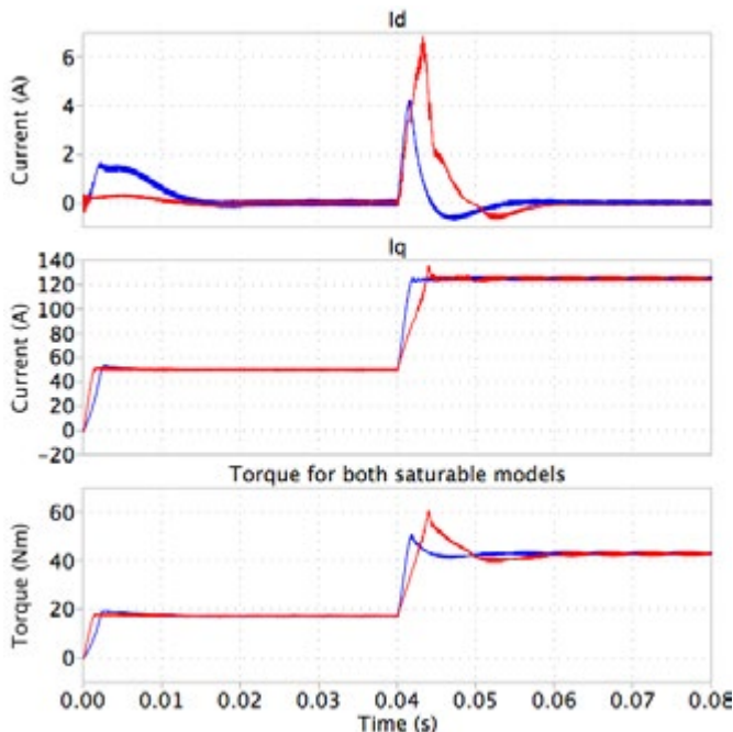
Figure 5: Transient response of i_d , i_q , and torque for a machine with heavy cross-saturation modeled with analytical functions (blue) and look-up tables (red)
