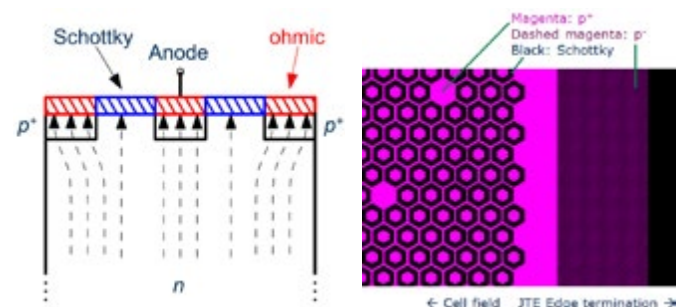
Figure 2: 1200 V thinQ!™ SiC Schottky diode generation 5 design. MPS (merged-pin-Schottky) structure combines the shielding of the electric field from the Schottky barrier and an increased surge current capability by hole injection. Dashed lines (left) show current density at higher currents. Cell design (right) of an optimized cell structure with hexagonal p^+ islands.
