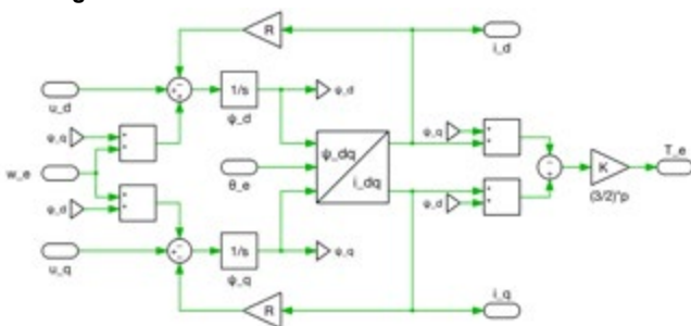
Figure 1: Implementation for the flux-based PMSM model [5]
