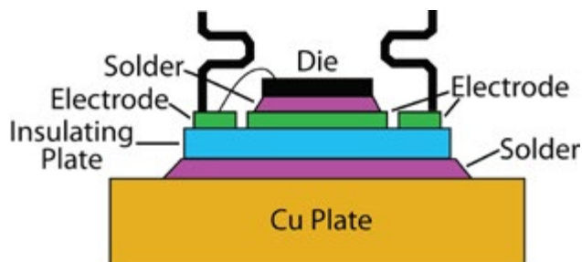
Figure 1: Diagrammatic side view of a GTO, Thyristor or IGBT module
