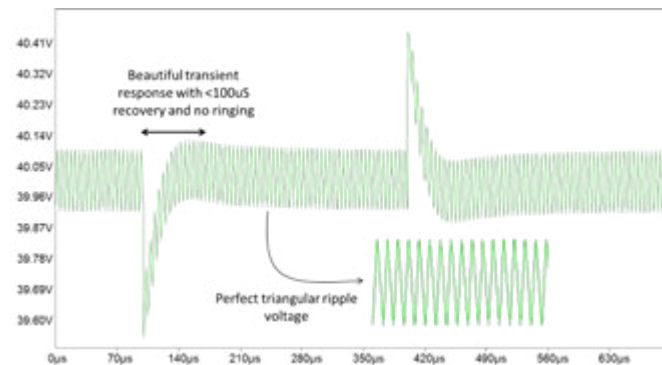
Figure 2: Type III compensator is performing very well
