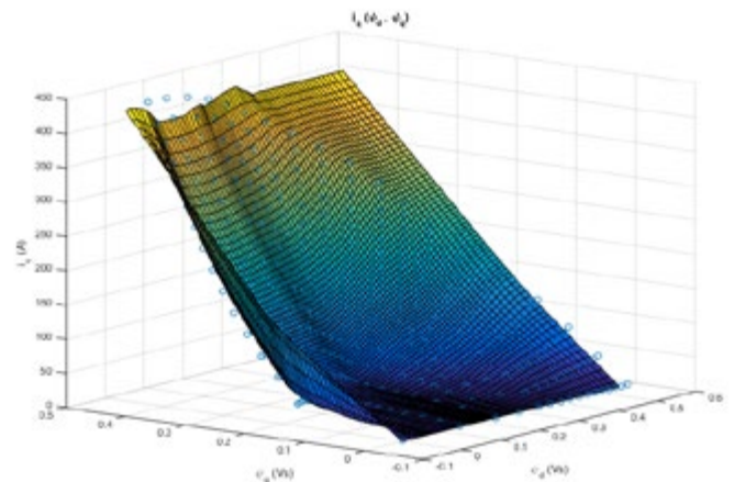
Figure 4: Look-up table generated for machine with high cross-saturation effects (surface: look-up table, dots: FEA data)>
