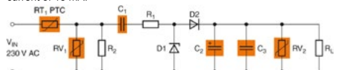
Figure 2: Simple capacitive power supply
