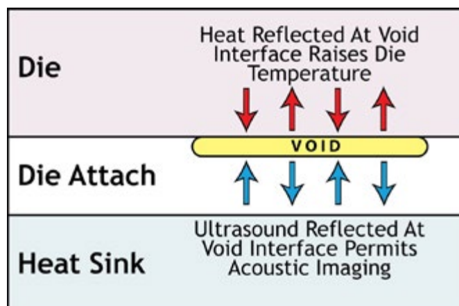
Figure 2: Any gap-type anomaly reflects heat (top), but also reflects the ultrasound that images the anomaly (bottom).
