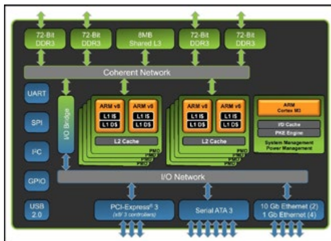
Picture 8: Block Diagram of the X-Gene 2 Processor
