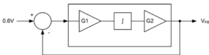
Figure 7: Control loop for regulating the LED current begins by maintaining the feedback voltage V_{FB} at 0.6V.
