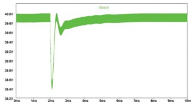
Figure 7: The spice simulation of the step response
