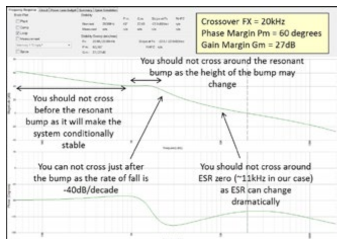
Figure 1: Optimally compensated voltage mode power supply with a Type III compensator using our WDS software
