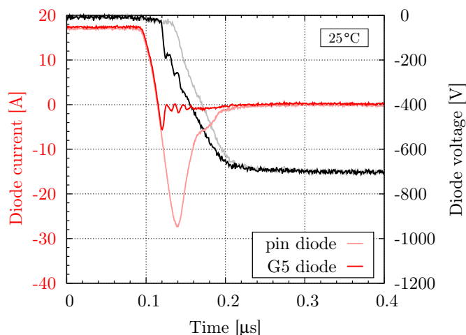
Figure 1: Reverse recovery behavior of a fast state of the art 1200 V Si-pin diode and SiC Schottky diode generation 5 (G5). V_{DC}=700 V, switch: 1200 V IGBT, di/dt=1300 A/ \mu s, losses: 50 \mu Ws for G5, 190 \mu Ws for Si-pin diode. Reverse voltage applied to the diode is represented in black curves.
