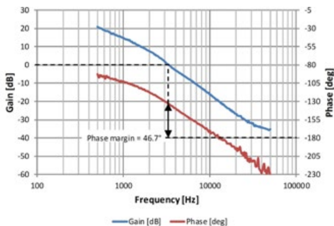
Figure 10: The Bode plot of the LED driver circuit with the current regulation confirms the circuit has sufficient phase margin to guarantee stable operation.
